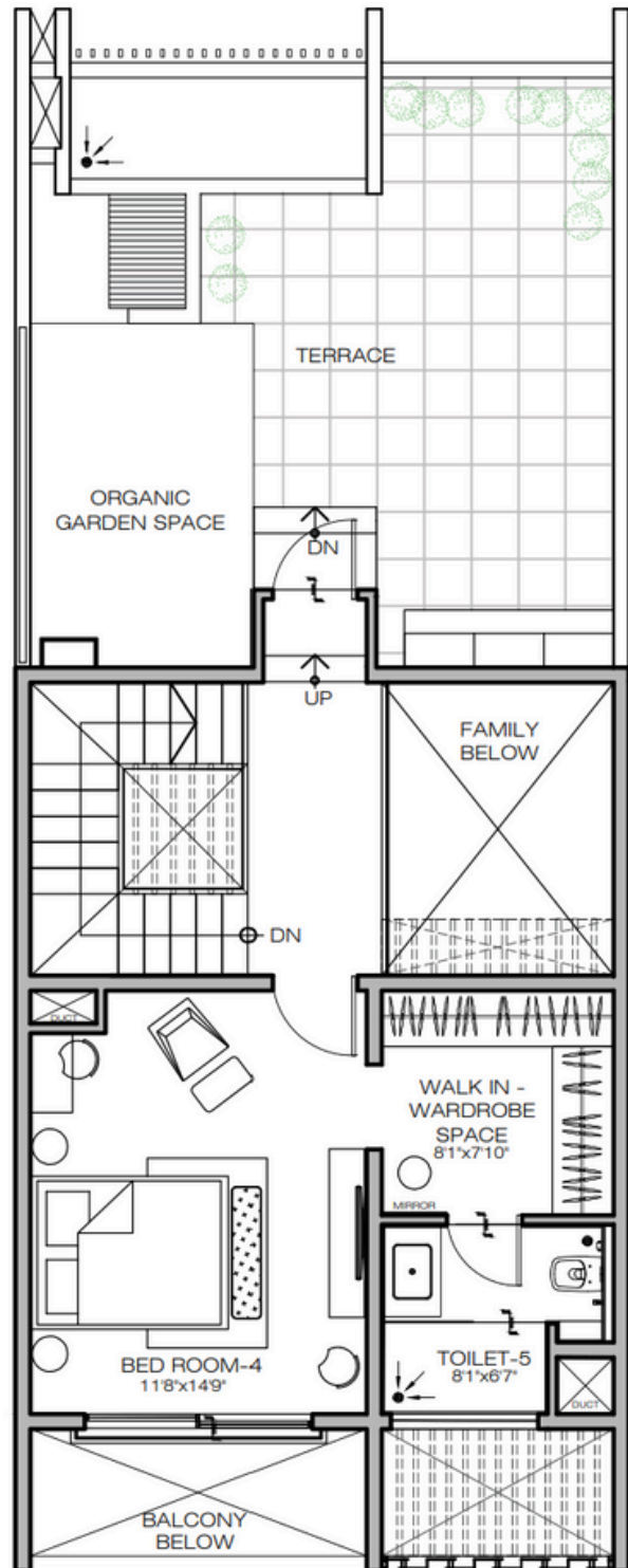
Third Floor Plan
