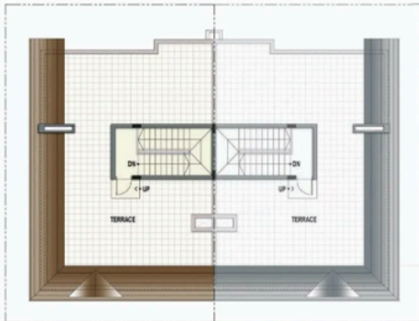
TERRACE FLOOR - VILLA TYPE-A
