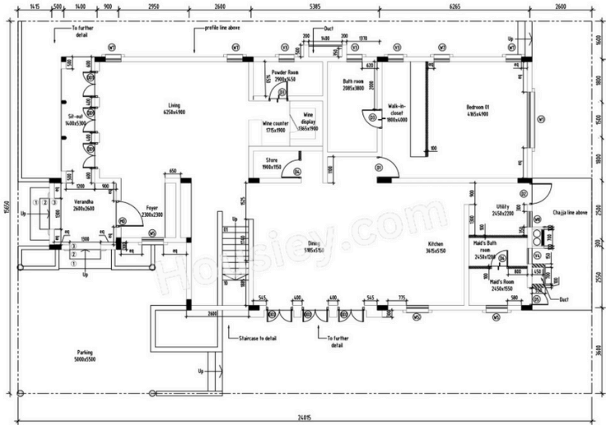
01 Ground Floor plan - Block-A Scale 1/75
